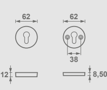
Diana Premium Rozeta
