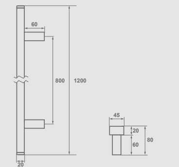
Amsterdam Prosta 120 cm
