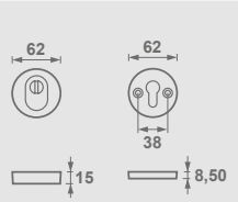
Diana Flex Premium Rozeta
