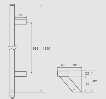
Amsterdam Skos 150 cm
