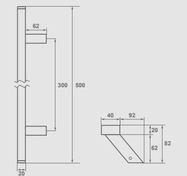
Amsterdam Skos 50 cm
