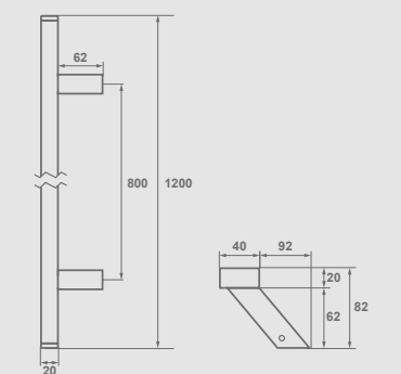
Amsterdam Skos 120 cm
