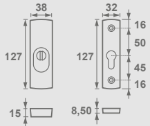
Solid Flex Premium Rozeta
