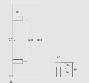
Amsterdam Prosta 80 cm
